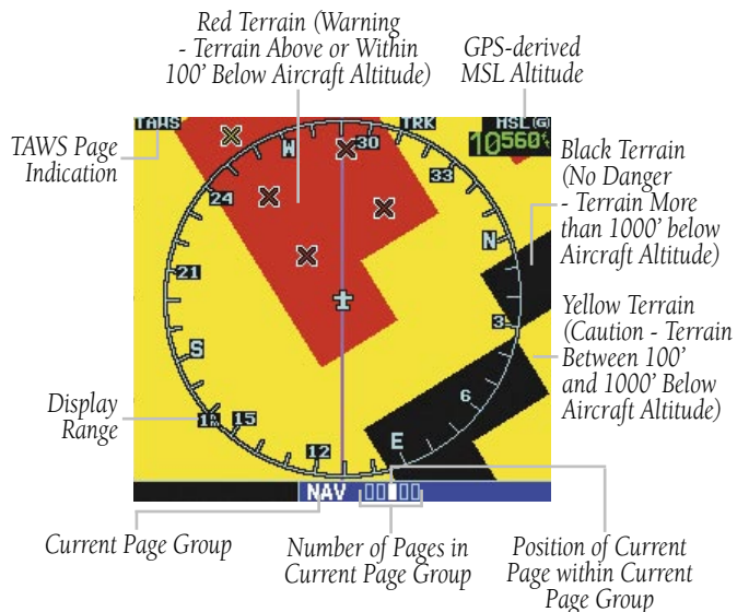
Figure 3-34 TAWS Page
